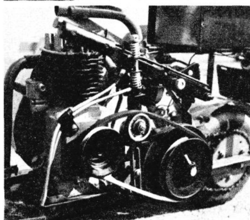
Above: Gas tank feeds motor by gravity. Dome shaped gadget near wheel is generator. Right: Clutching arrangement is operated by idler pulley (center) which raises and lowers to engage or disengage driver pulleys. Wheel itself (with sprocket) is in turn driven by chain from sprocket on pulley shaft,
